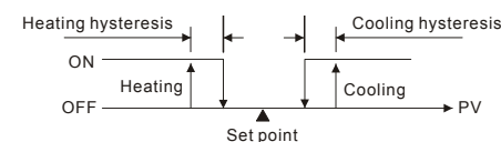
Figure 1: Output operation when in On/Off control
