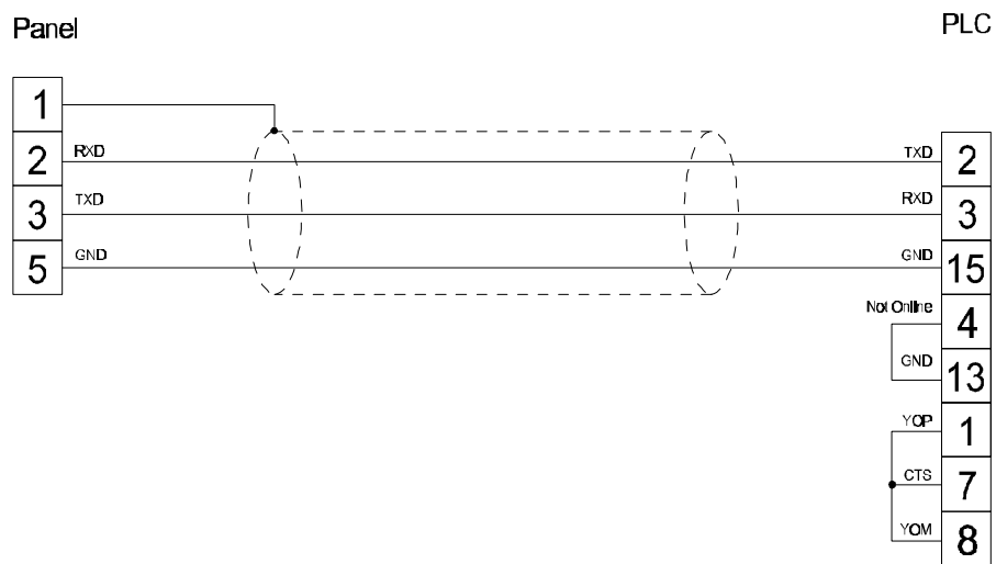
Figure 1. Cable diagram
