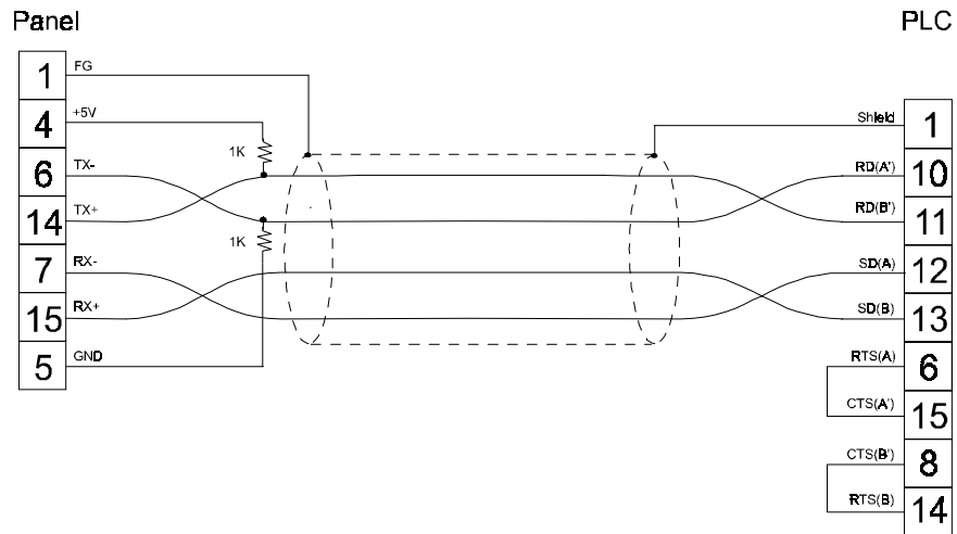
figure 1. Cable diagram
