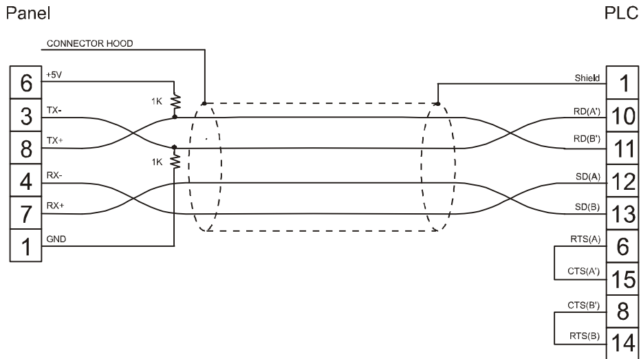
figure 1. Cable diagram
