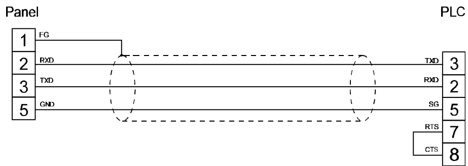
figure 1. Cable diagram
