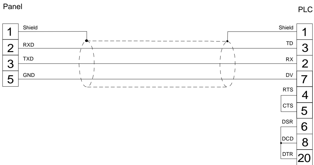
figure 1. Cable diagram
