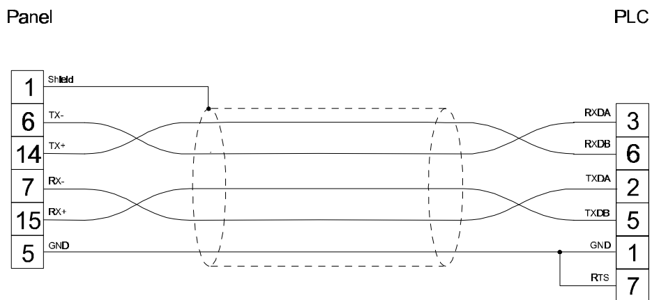
figure 1. Cable diagram
