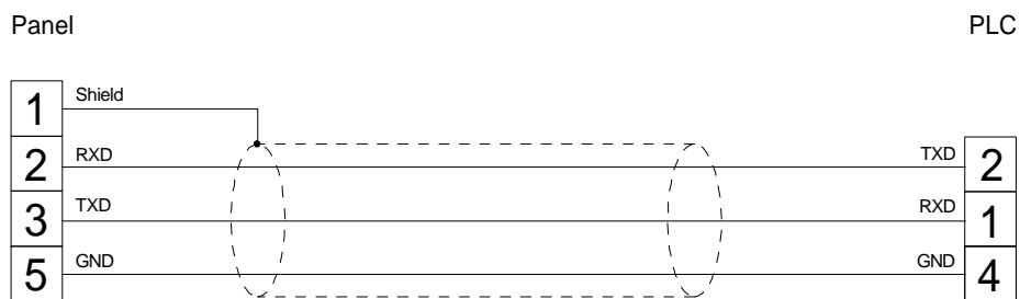
Figure 1. Cable diagram
