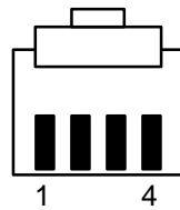
Figure 2. PLC Connector (front view)
