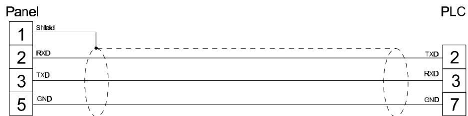
figure 1. Cable diagram
