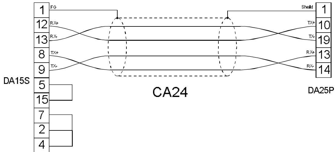
figure 1. Cable diagram
