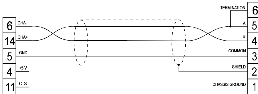
figure 1. Cable diagram
