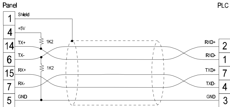
Figure 1. Cable diagram
