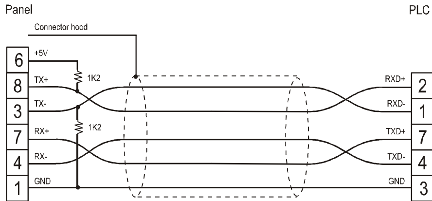
Figure 1. Cable diagram
