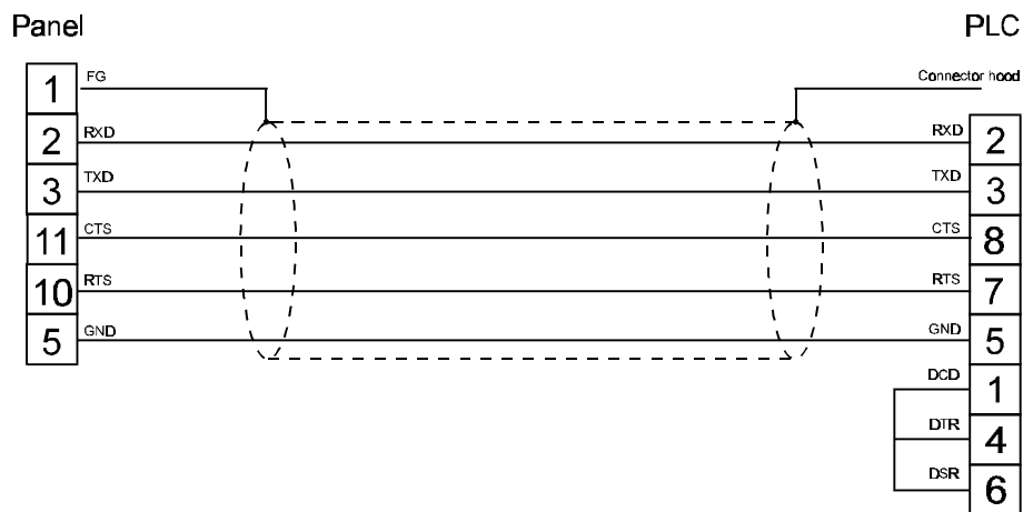
figure 1. Cable diagram
