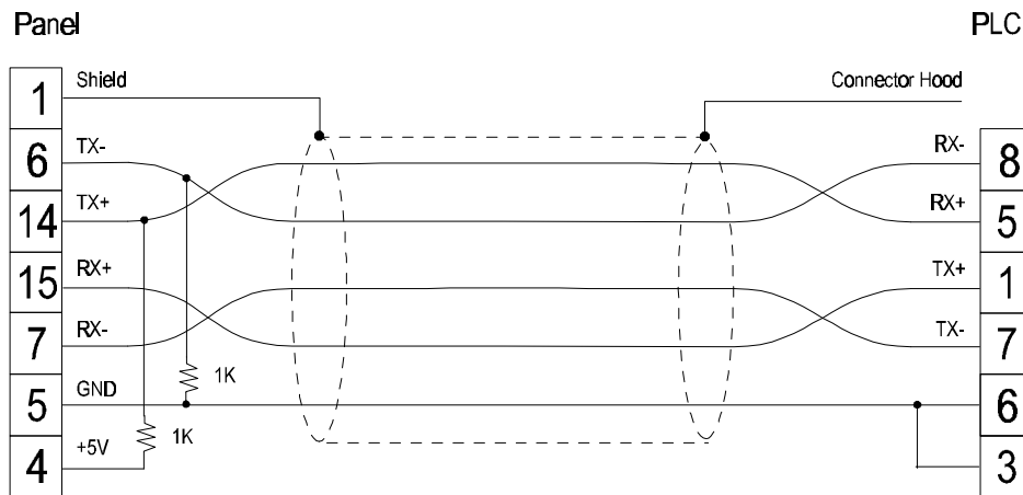
Figure 1. Cable diagram
