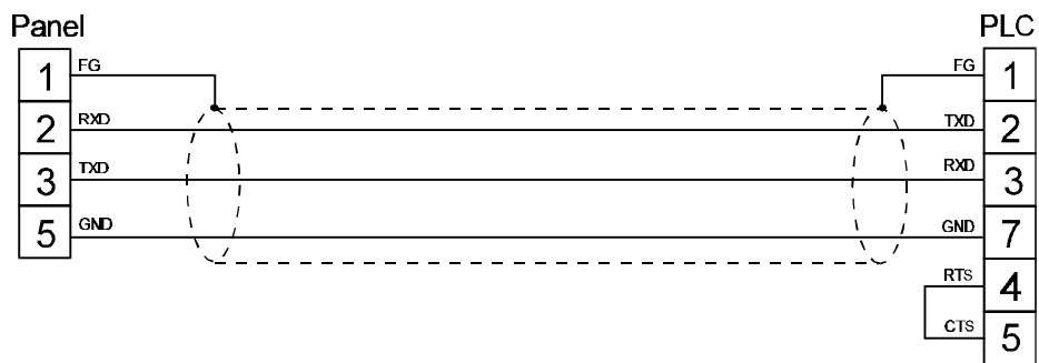
figure 1. Cable diagram
