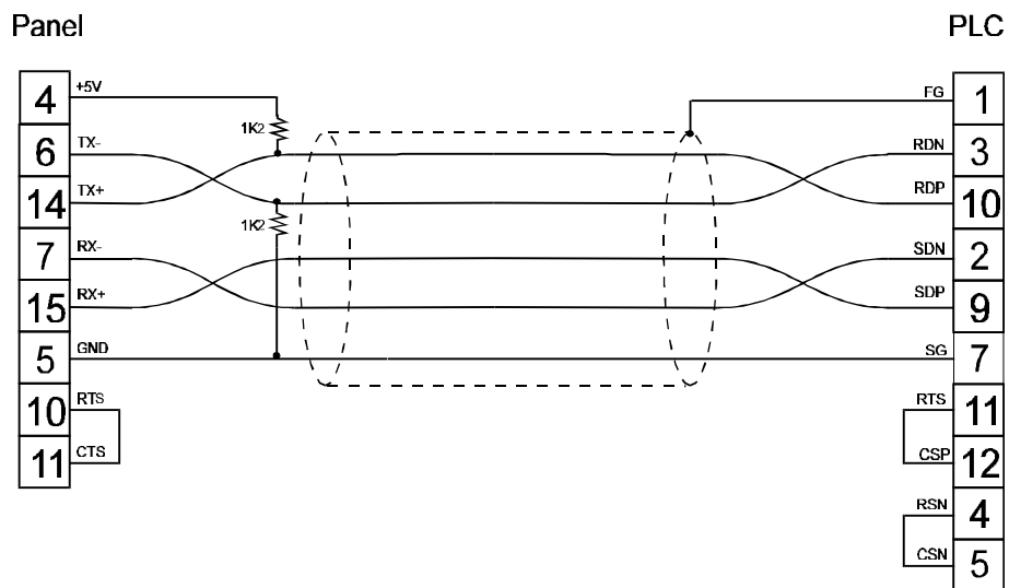
figure 1. Cable diagram
