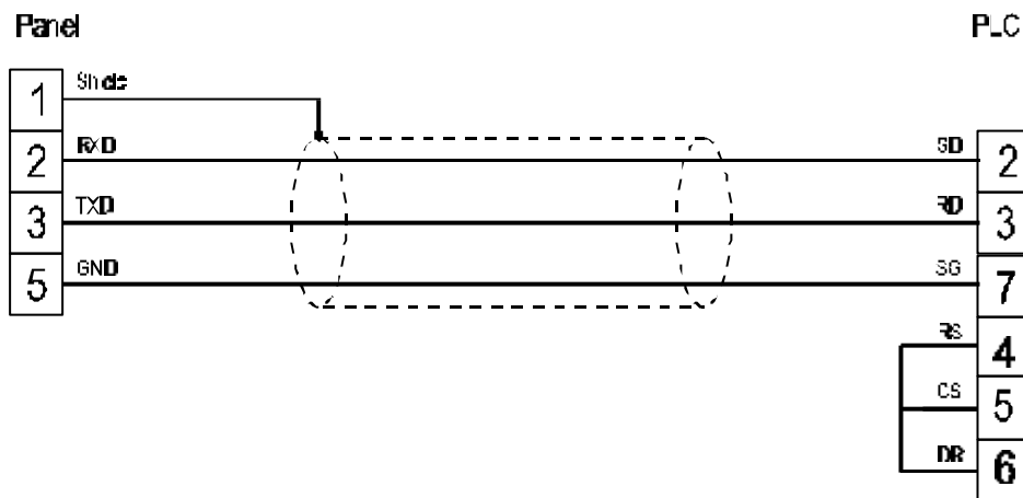
figure 1. Cable diagram
