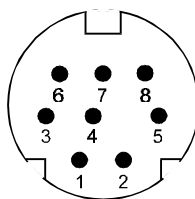
figure 2. Connector front view (pin side)
