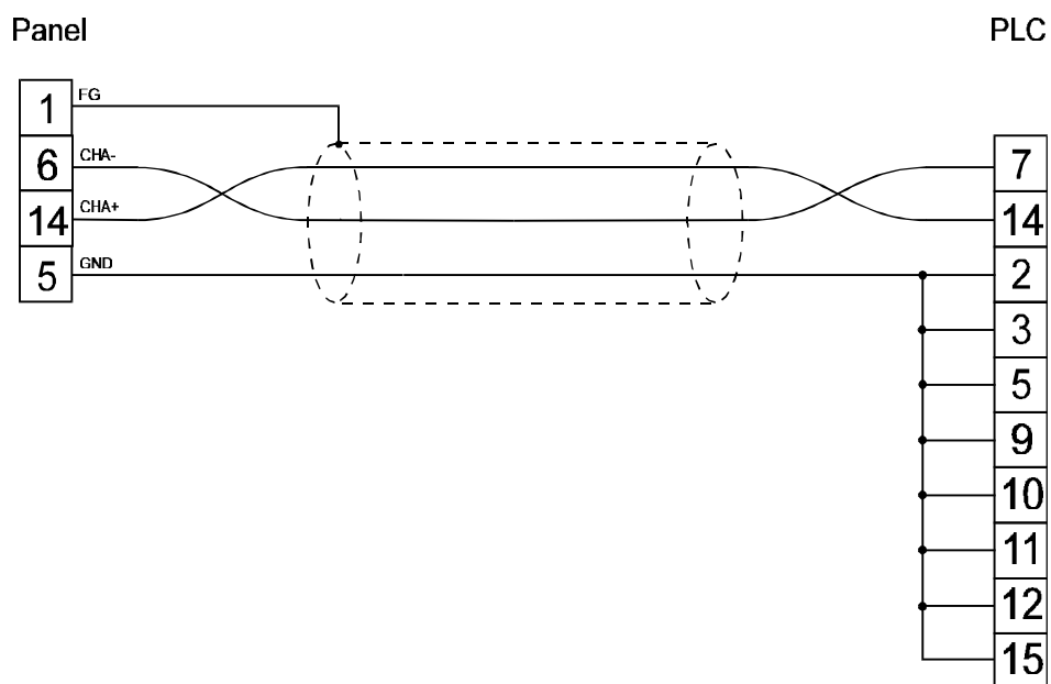
figure 1. Cable diagram
