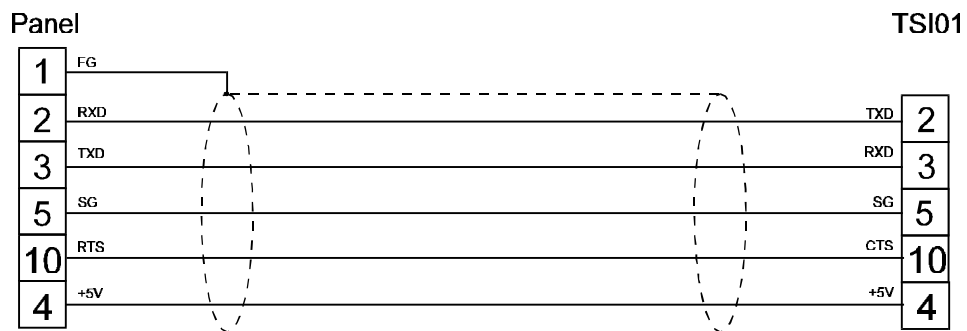
figure 1. Cable diagram
