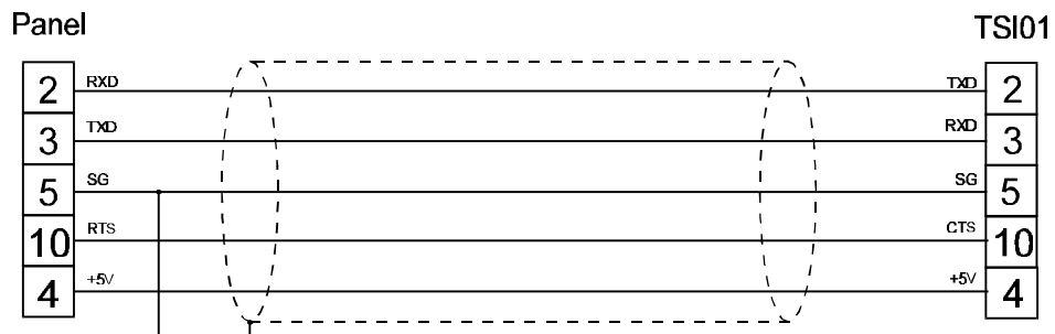
figure 1. Cable diagram
