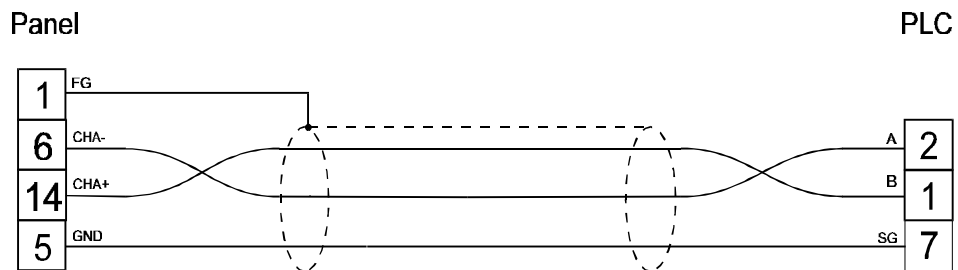
figure 1. Cable diagram
