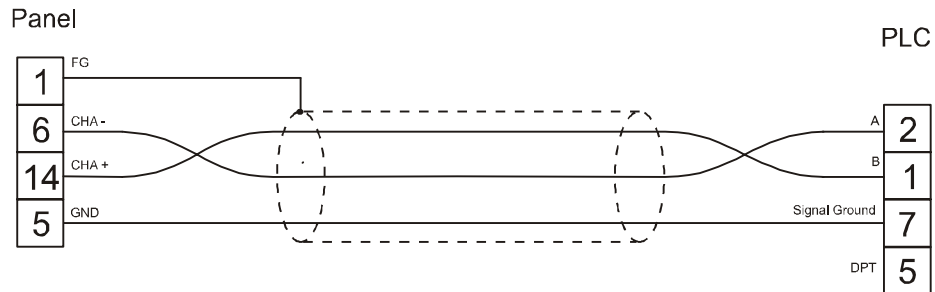
figure 1. Cable diagram
