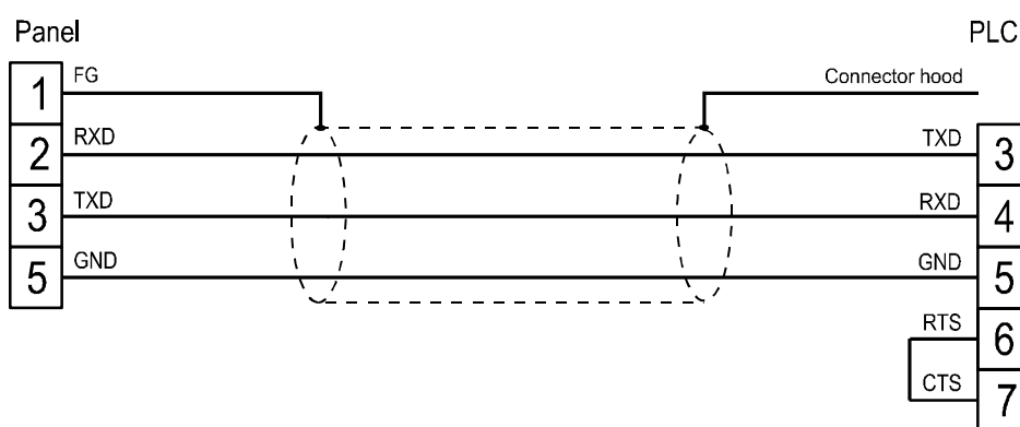
Figure 1. Cable diagram
