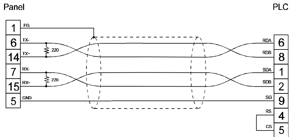
figure 1. Cable diagram
