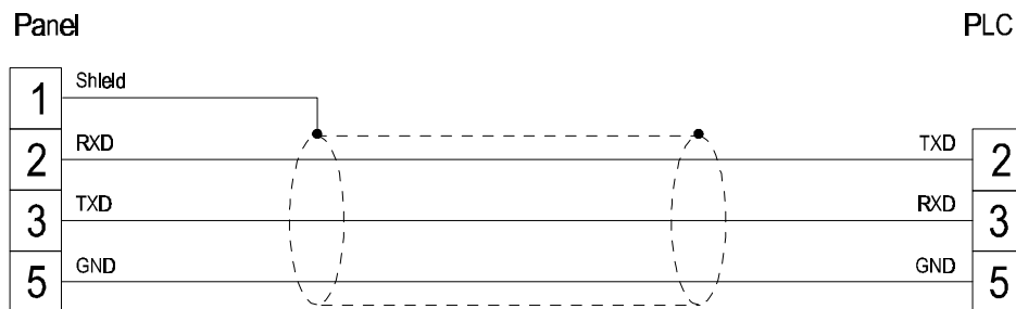
Figure 1. Cable diagram
