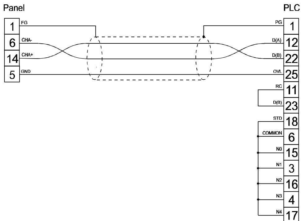
figure 1. Cable diagram
