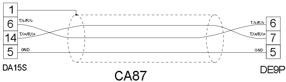
figure 1. Cable diagram
