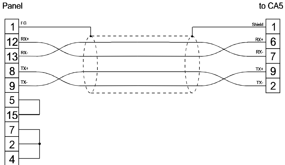
figure 1. Cable diagram
