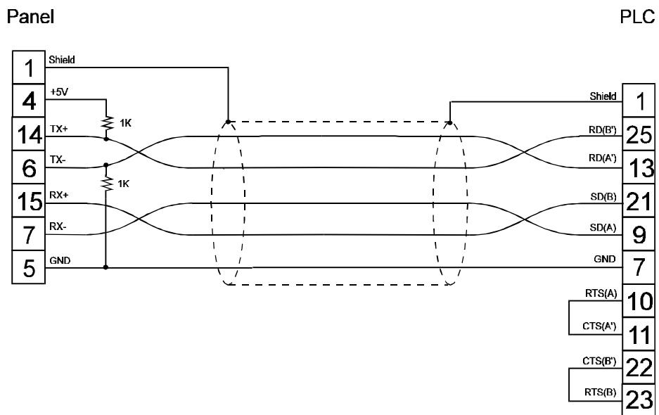
figure 1. Cable diagram
