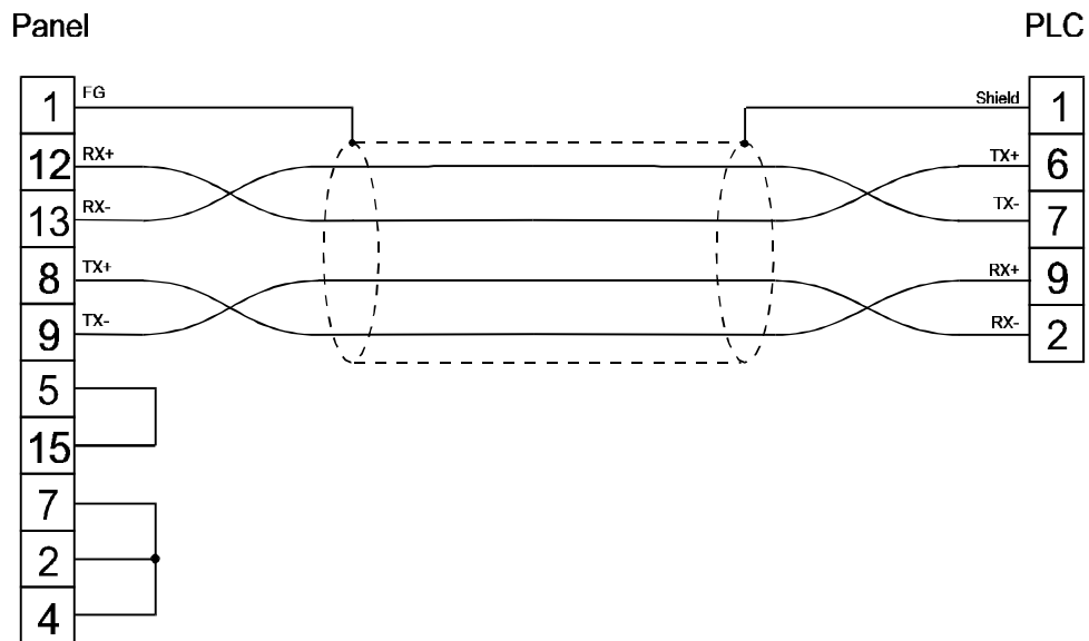
figure 1. Cable diagram
