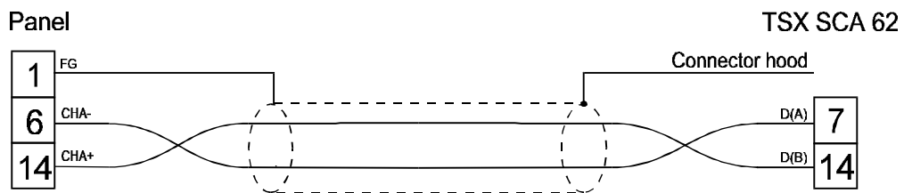
figure 1. Cable diagram
