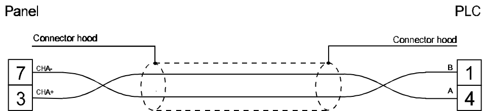
figure 1. Cable diagram
