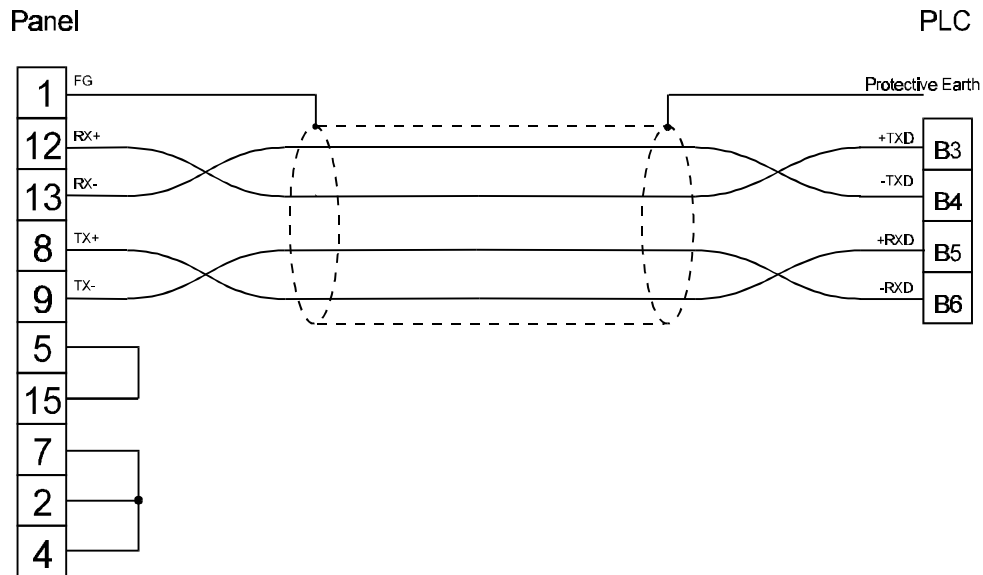
figure 1. Cable diagram
