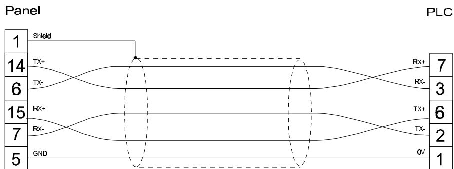
Figure 1. Cable diagram
