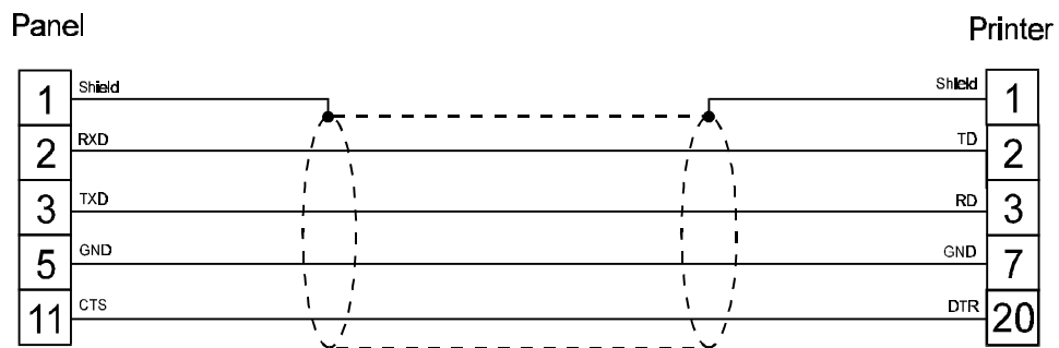
figure 1. Cable diagram
