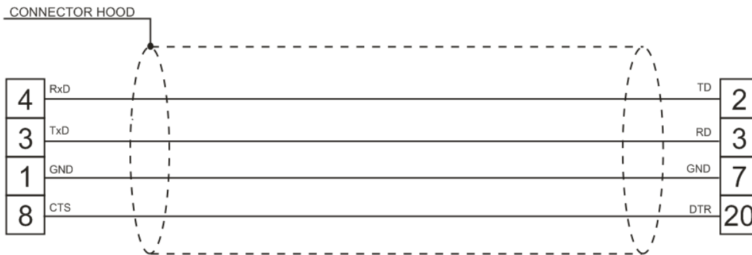
Figure 1. Cable diagram
