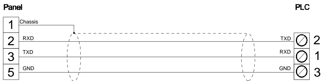
Figure 1. Cable diagram
