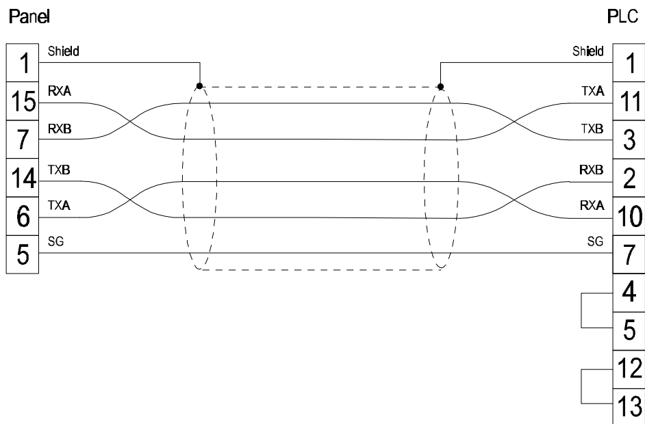
Figure 1. Cable diagram
