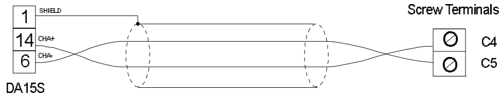
figure 1. Cable diagram
