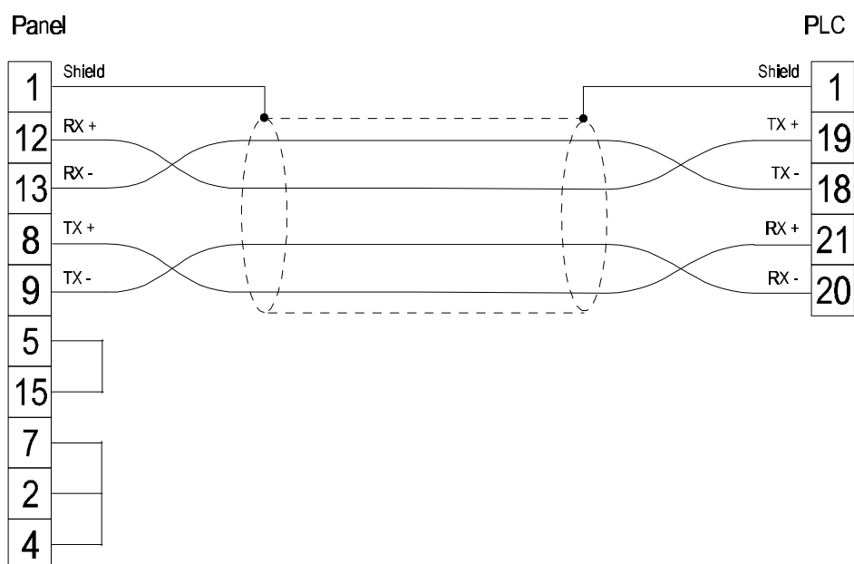
Figure 1. Cable diagram
