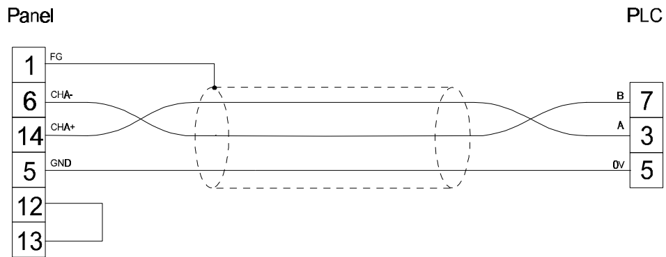
figure 1. Cable diagram
