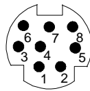
figure 2. PLC connector - pin side
