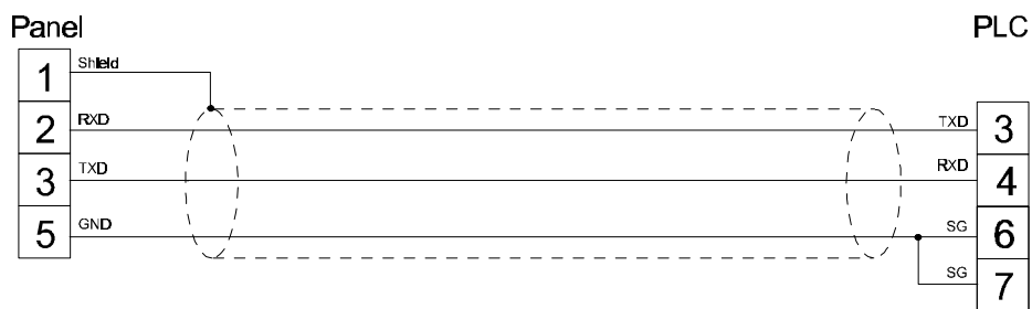
figure 1. Cable diagram
