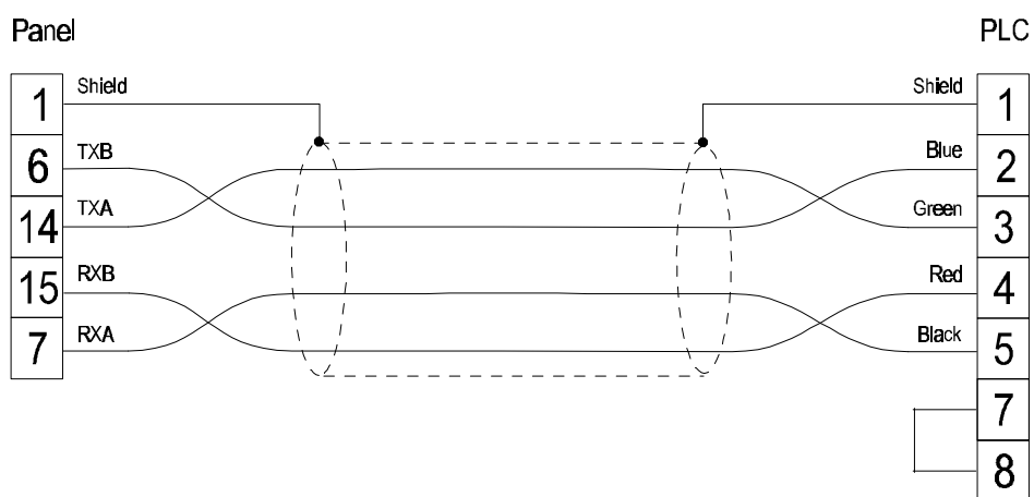
Figure 1. Cable diagram
