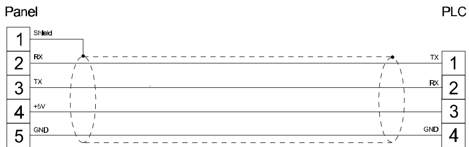
figure 1. Cable diagram
