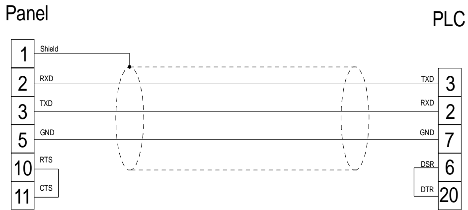
figure 1. Cable diagram
