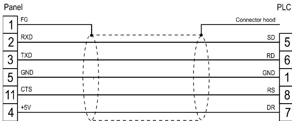
Figure 1. Cable diagram
