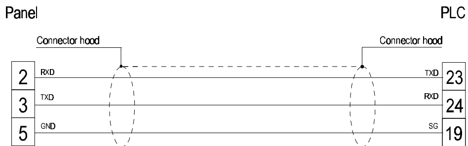
figure 1. Cable diagram
