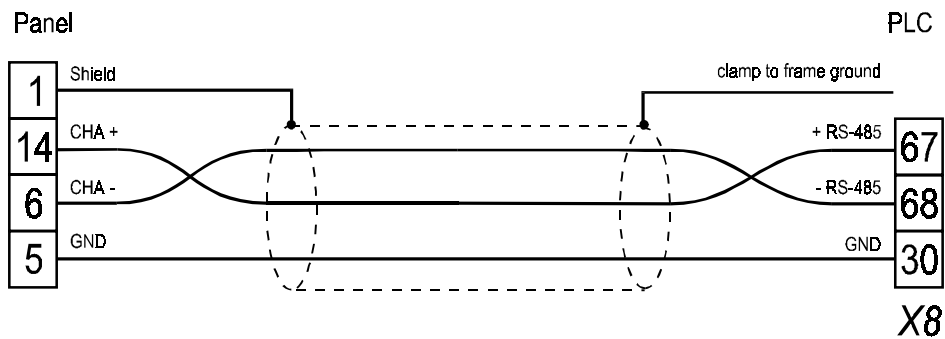
figure 1. Cable diagram
